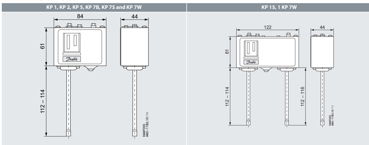
Figure 1: KP with top cover
