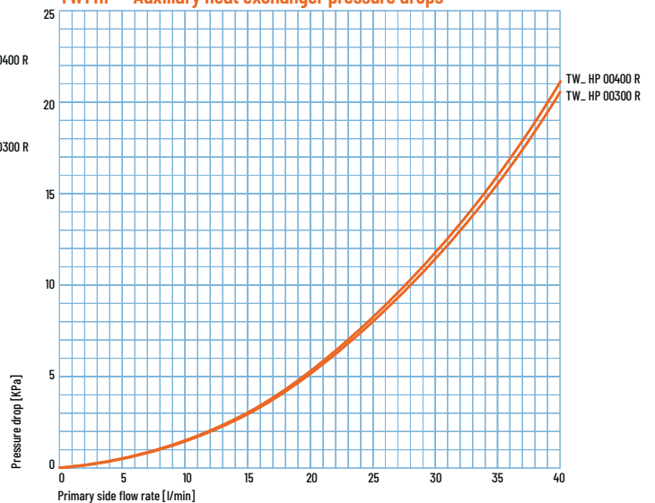
TW1 HP - Auxiliary heat exchanger pressure drops
