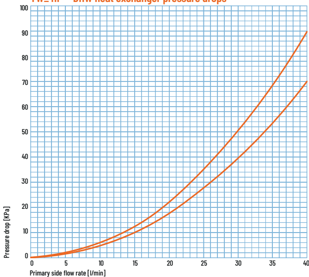
TW_HP - DHW heat exchanger pressure drops
