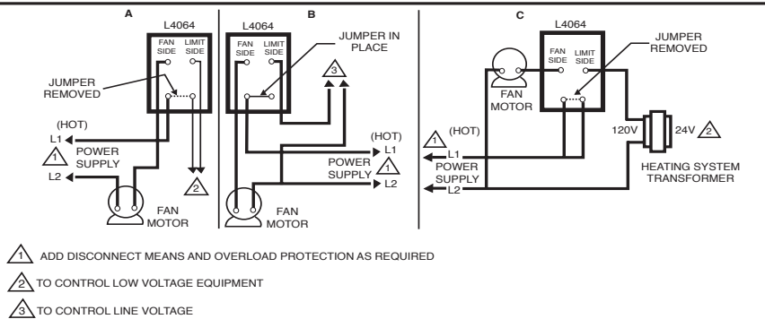
Fig. 9 - A: Limit in low voltage circuit.
